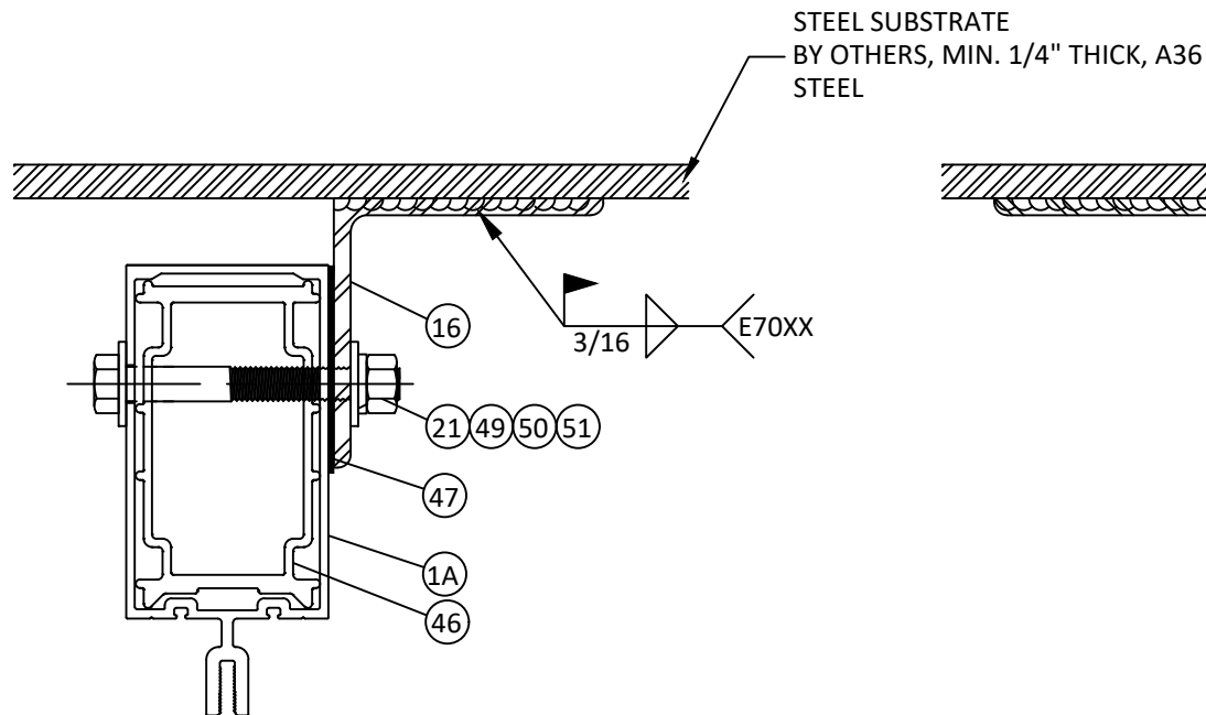
A 18 HORIZONTAL SECTION DEAD LOAD ANCHOR AT JAMB
