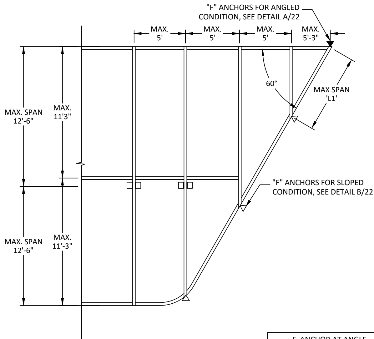
TYPICAL ELEVATION SLOPED & ANGLED CONDITION
