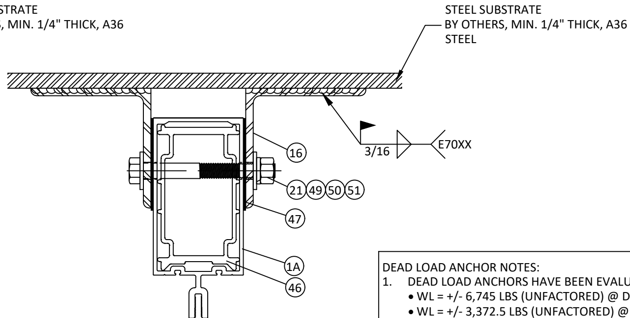
B 18 HORIZONTAL SECTION DEAD LOAD ANCHOR AT VERTICAL MULLION
