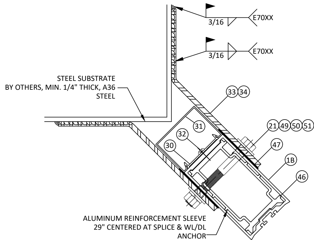
B HORIZONTAL SECTION 6 OUTSIDE CORNER WL ANCHOR
