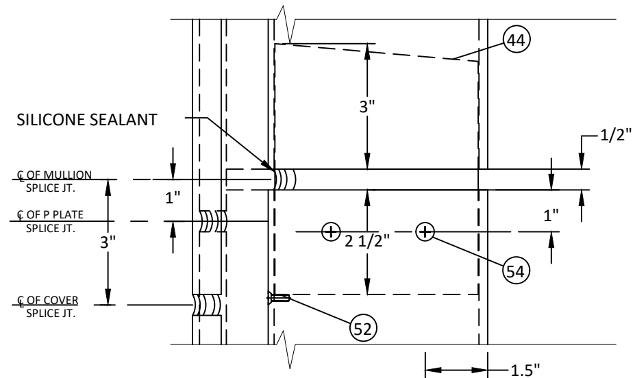
F 17 VERTICAL SECTION MULLION SPLICE
