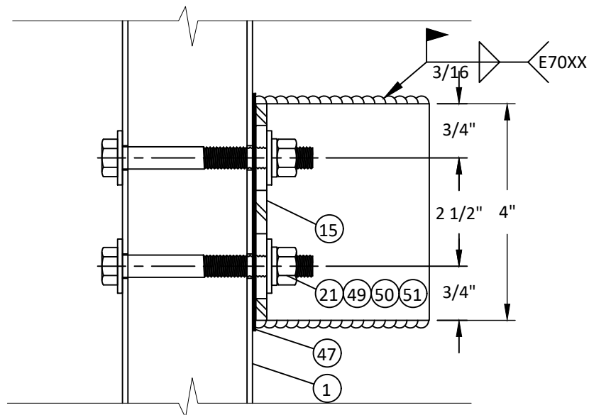
D 17 EXTERIOR VIEW WIND LOAD ANCHOR AT JAMB
