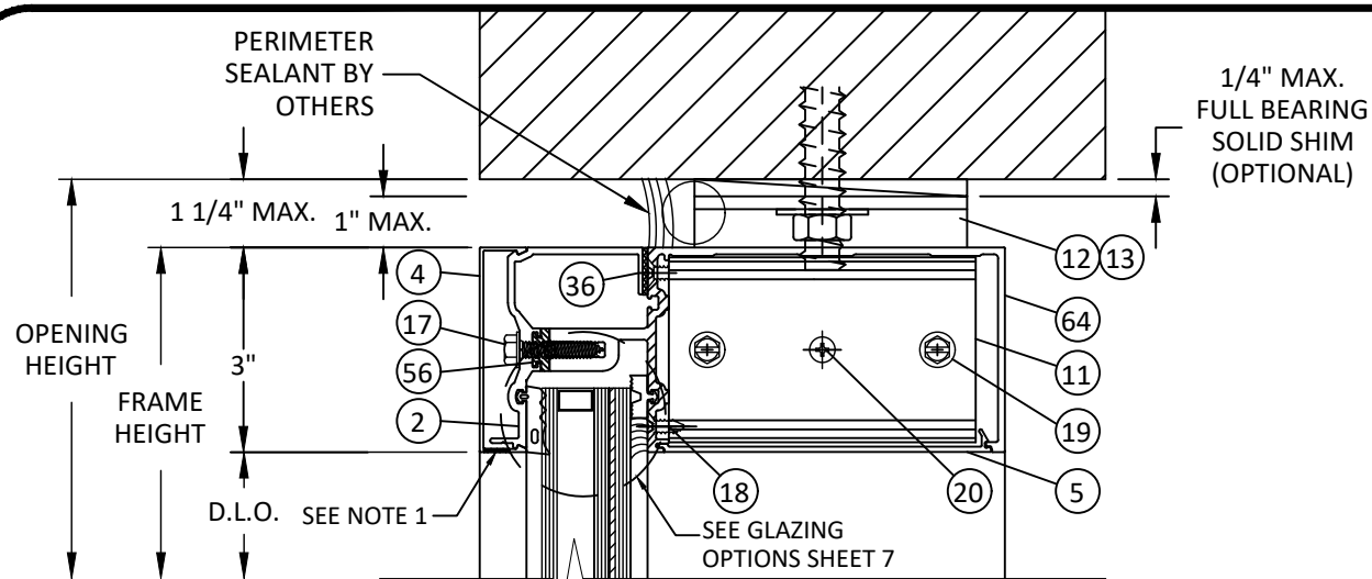
A 3 VERTICAL SECTION HEAD
