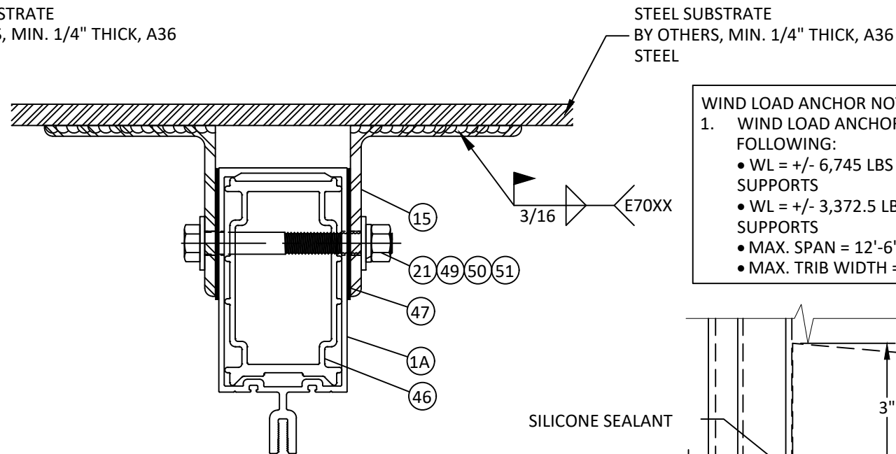
B 17 HORIZONTAL SECTION WIND LOAD ANCHOR AT VERTICAL MULLION
