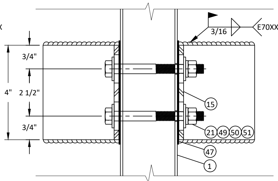
E 17 EXTERIOR VIEW WIND LOAD ANCHOR AT VERTICAL MULLION
