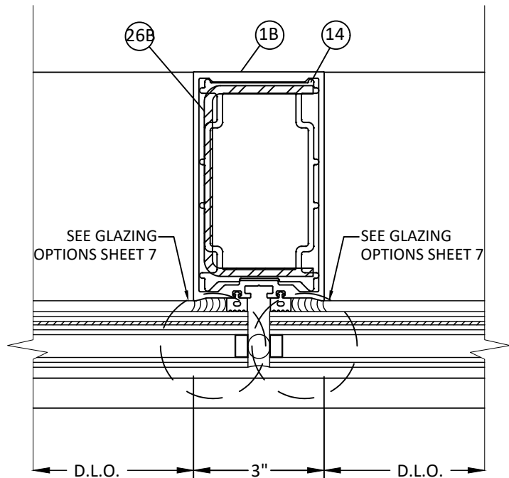
B 4 HORIZONTAL SECTION YHC 300 OG - VERTICAL MULLION STEEL REINFORCED
