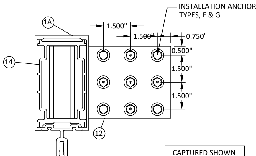
A 12 HORIZONTAL SECTION F-ANCHOR FOR WOOD SUBSTRATES
