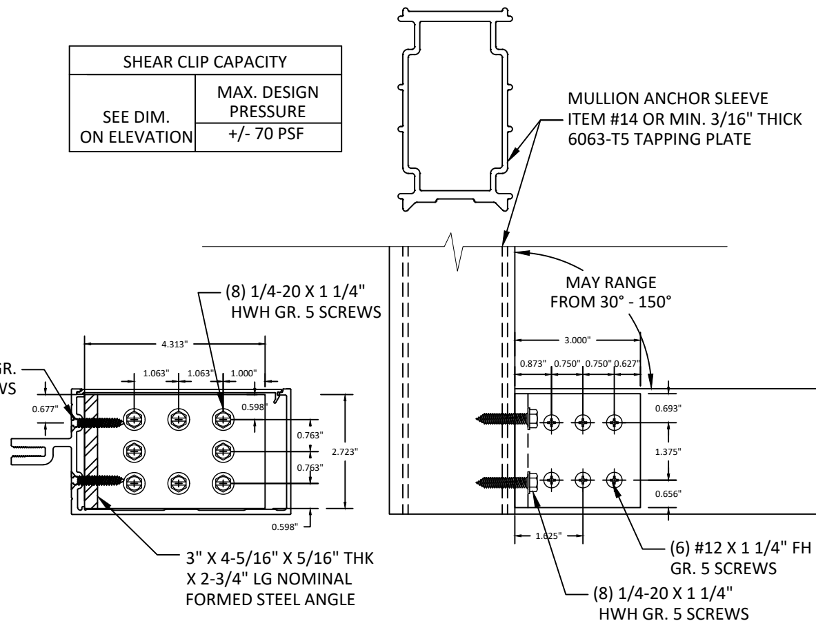
DETAIL SHEAR CLIP FORMED STEEL ANGLE
