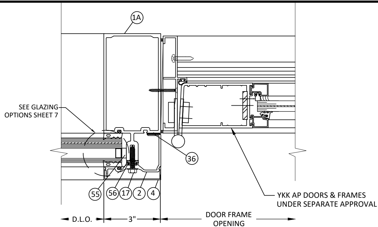
B 5 HORIZONTAL SECTION VERTICAL MULLION DOOR JAMB
