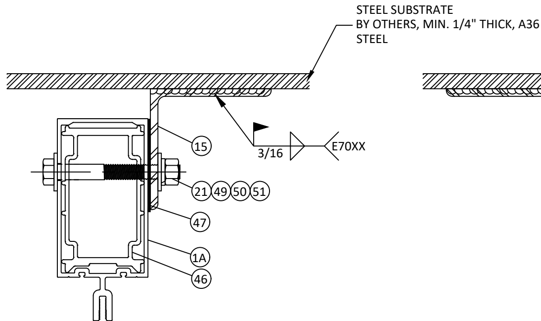
A 17 HORIZONTAL SECTION WIND LOAD ANCHOR AT JAMB
