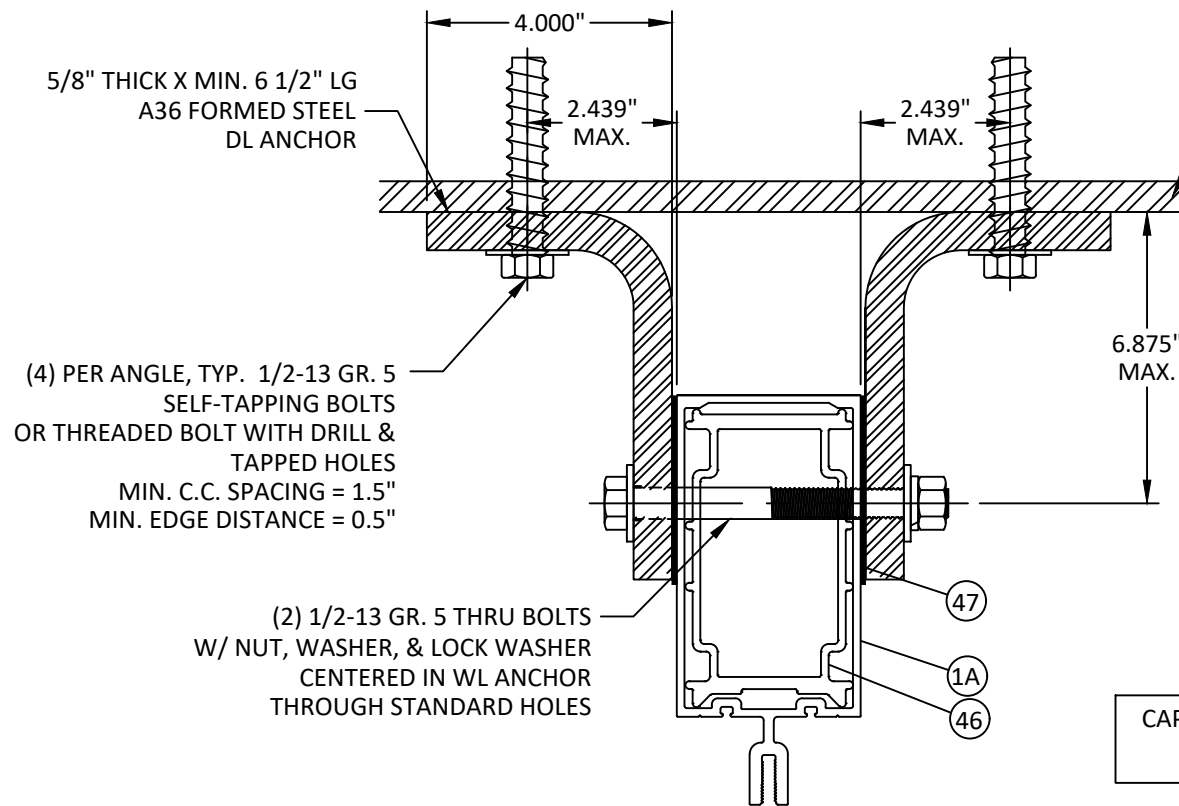
A HORIZONTAL SECTION 20 DEAD LOAD ANCHOR AT VERTICAL MULLION
