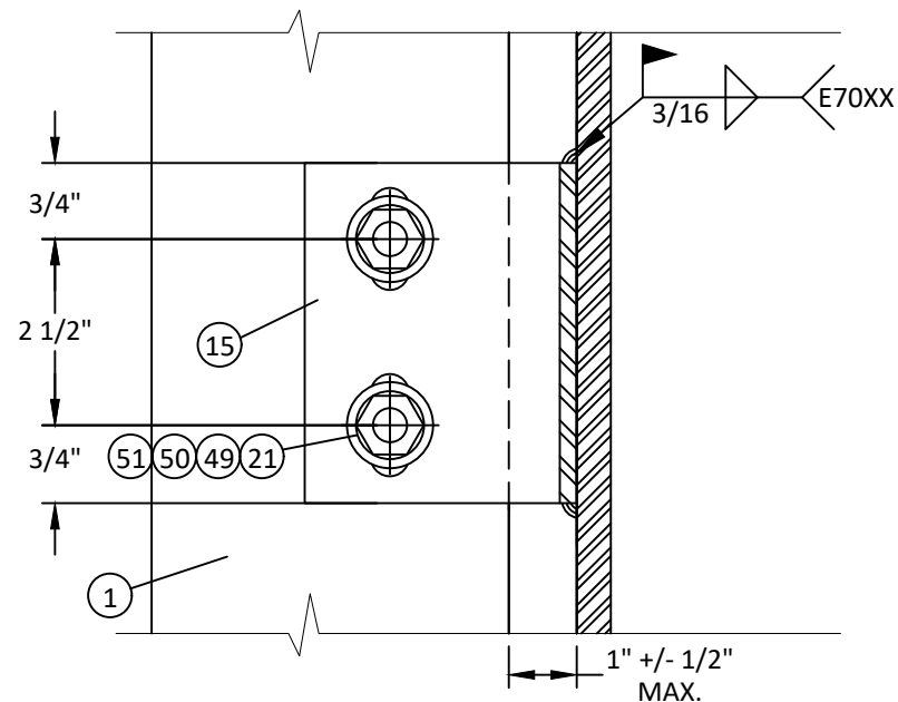
C 17 VERTICAL SECTION WIND LOAD ANCHOR STEEL SUBSTRATE
