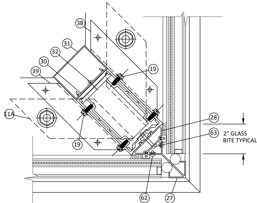
A HORIZONTAL SECTION 6 OUTSIDE CORNER TYPICAL
