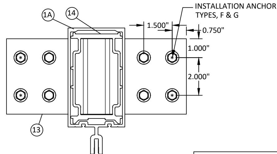
C 12 VERTICAL SECTION T-ANCHOR FOR WOOD SUBSTRATES
