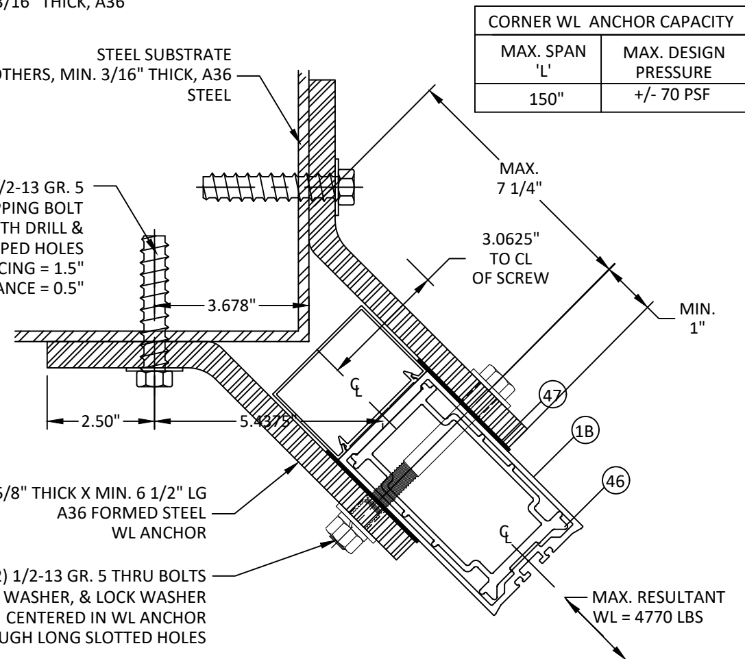
C HORIZONTAL SECTION 20 OUTSIDE CORNER WL ANCHOR
