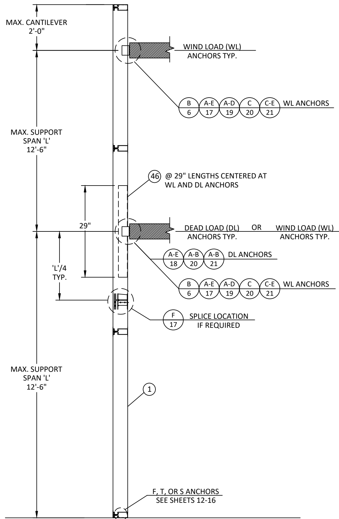
VERTICAL SECTION MULTI-SPAN TYP.
